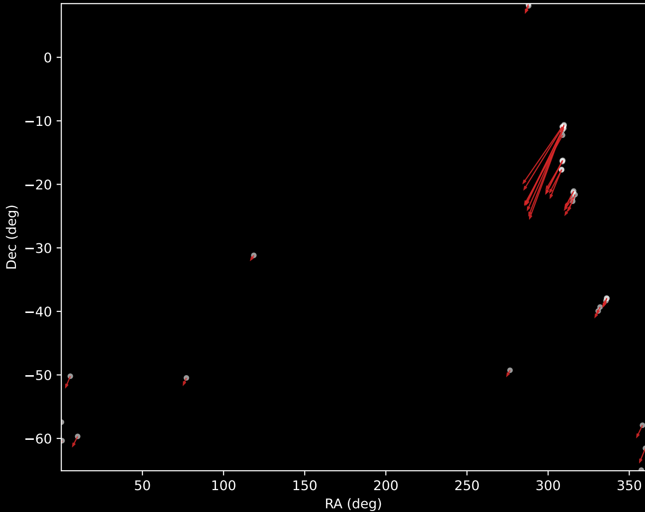
GALAH DR4 Cluster 66 Proper Motion Vectors (n=35)
