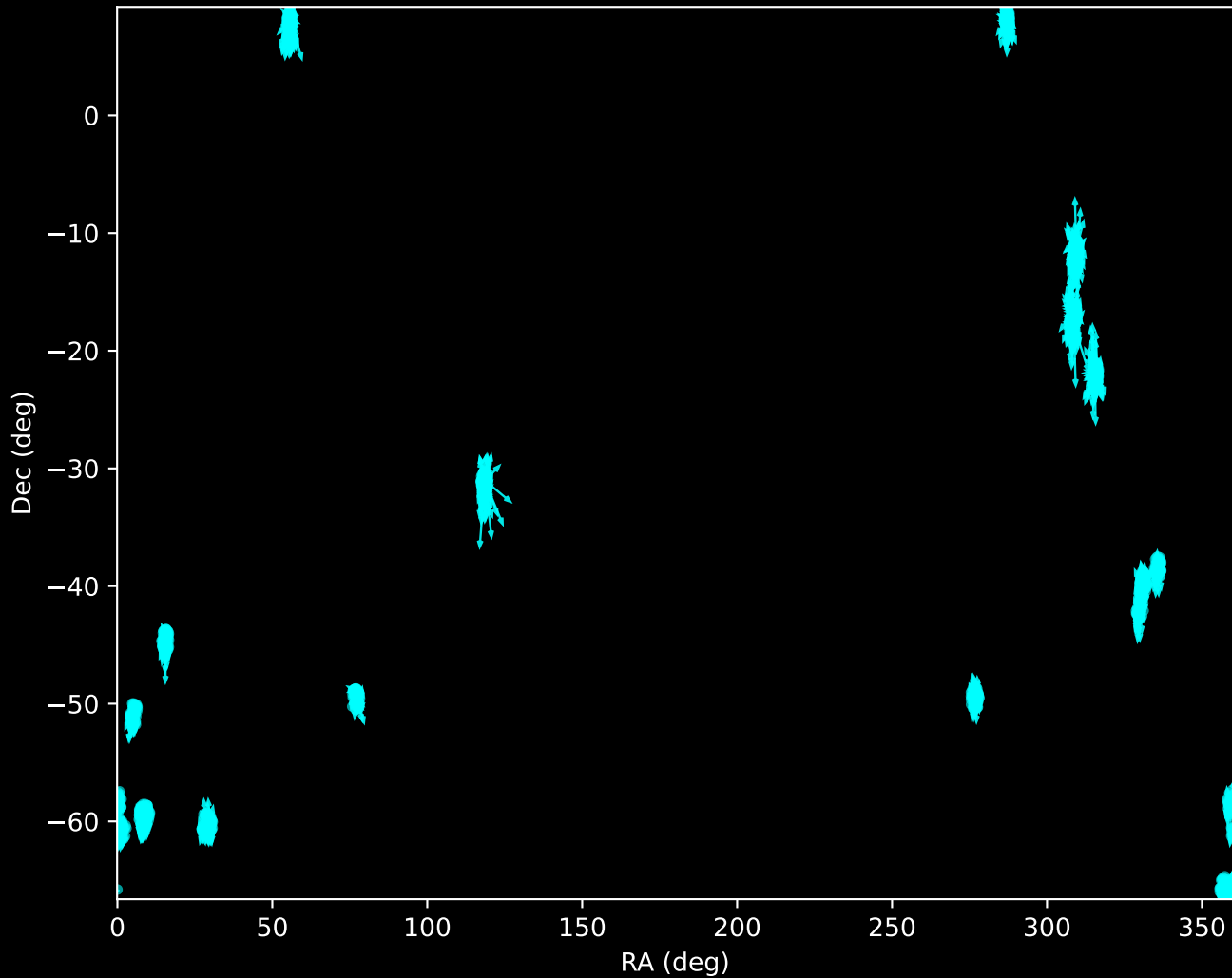
GALAH DR4 Noise Stream Proper Motion Vectors (n=1417)
