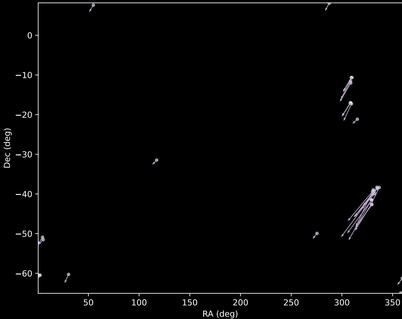
GALAH DR4 Cluster 109 Proper Motion Vectors (n=32)
