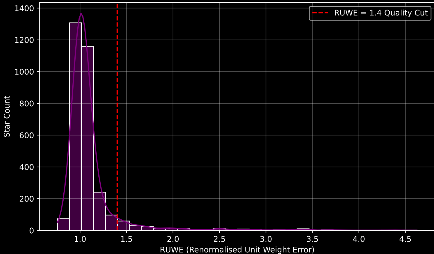
GALAH DR4 Field [-11] RUWE Distribution (n= 3108)
