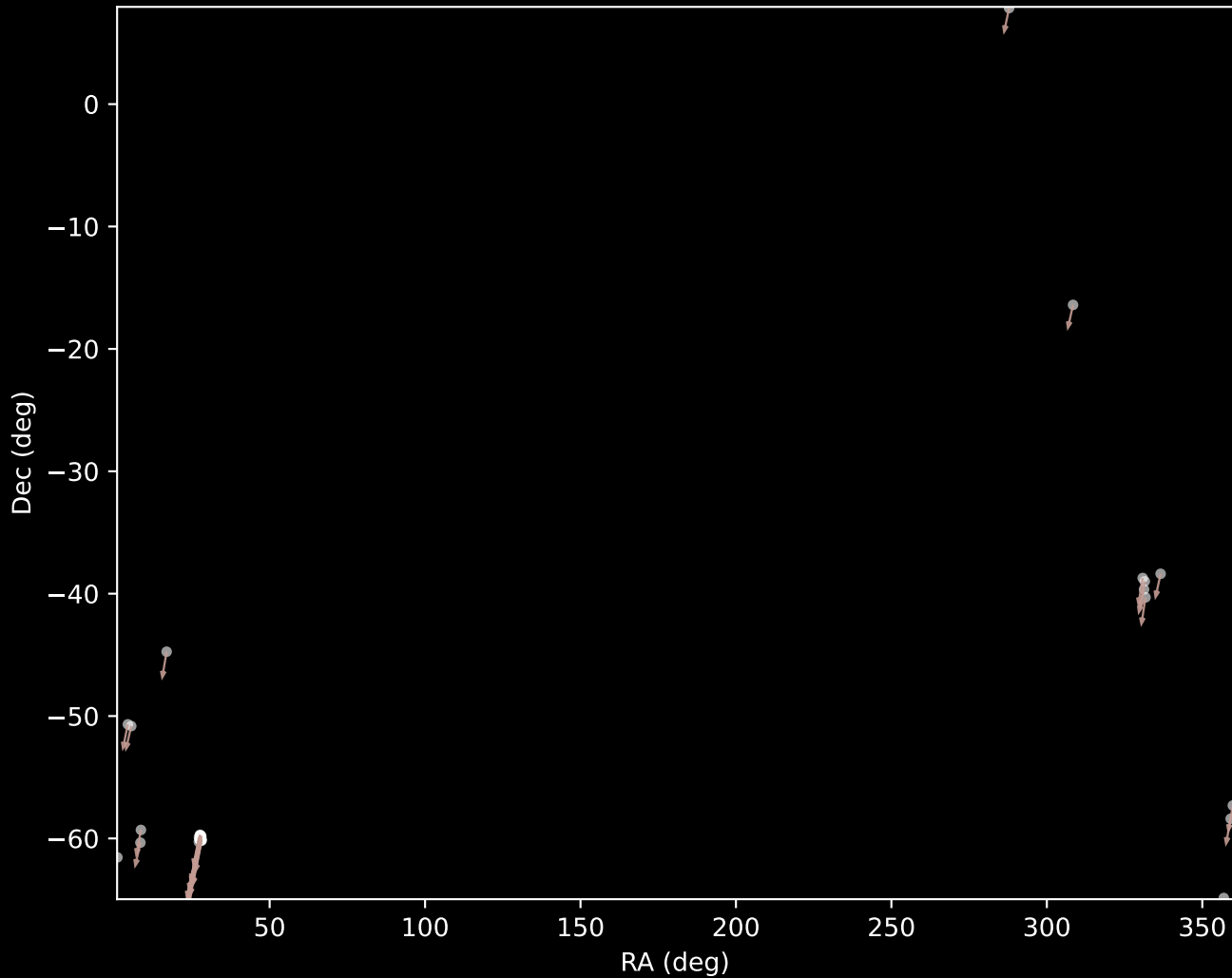
GALAH DR4 Cluster 171 Proper Motion Vectors (n=49)
