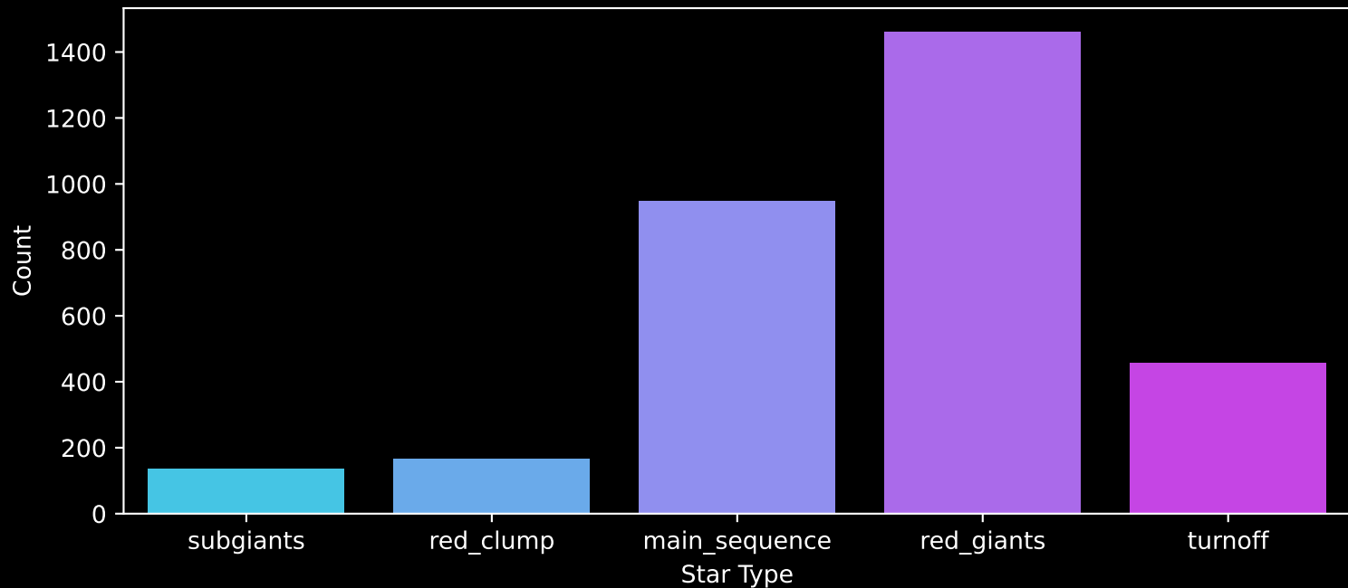
GALAH DR4 Field: [-11] Count plot of Star Type
