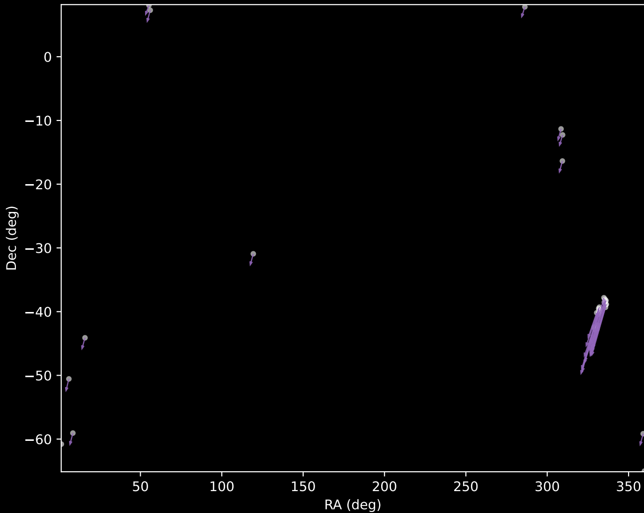
GALAH DR4 Cluster 128 Proper Motion Vectors (n=32)
