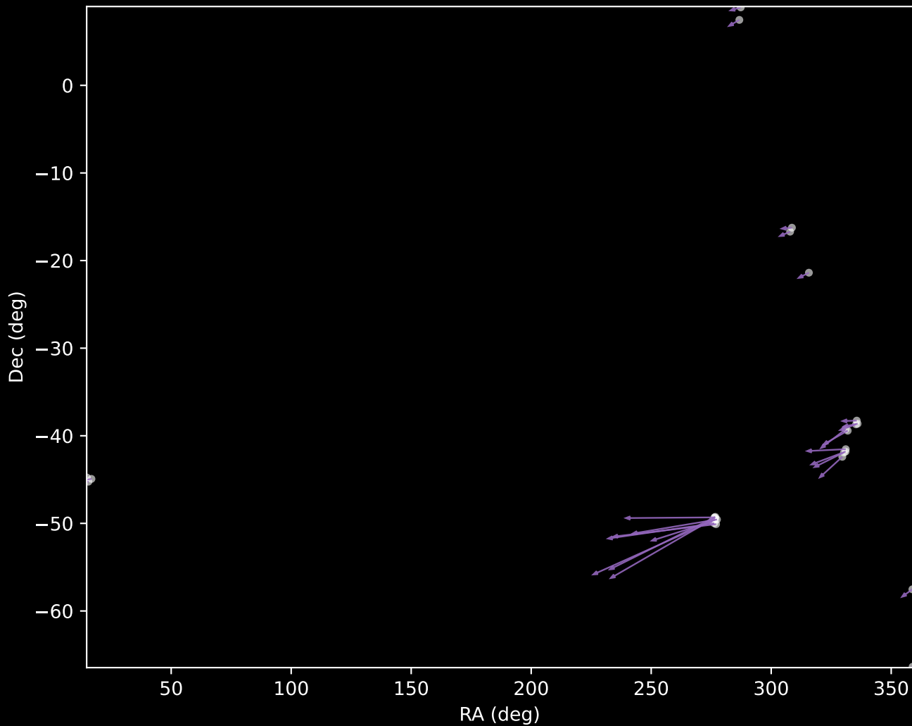
GALAH DR4 Cluster 108 Proper Motion Vectors (n=27)
